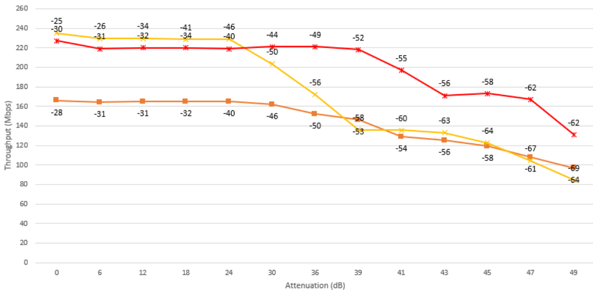
Band 2.4GHz: Download (Mbps) - STA 802.11AX 20MHz
