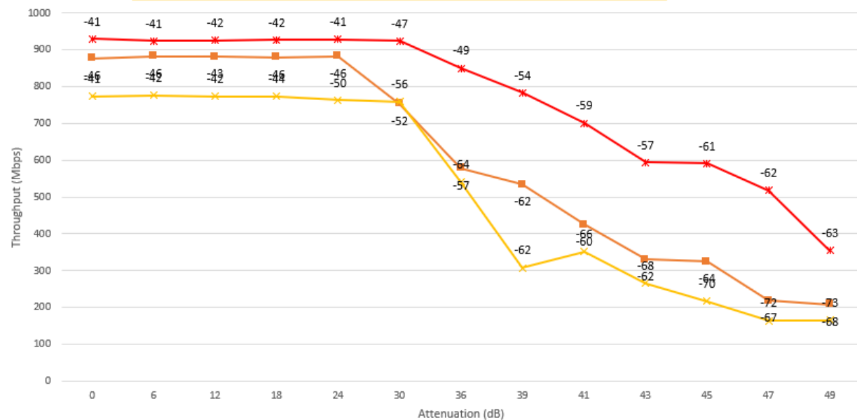
Band 5GHz: Upload (Mbps) - STA 802.11AX 80MHz
