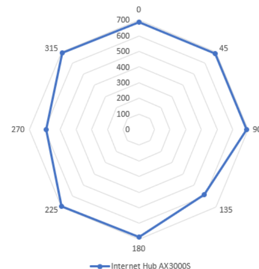
Spatial Consistency_5GHz_Download with STA's RSSI around -65 dBm to -70dBm
