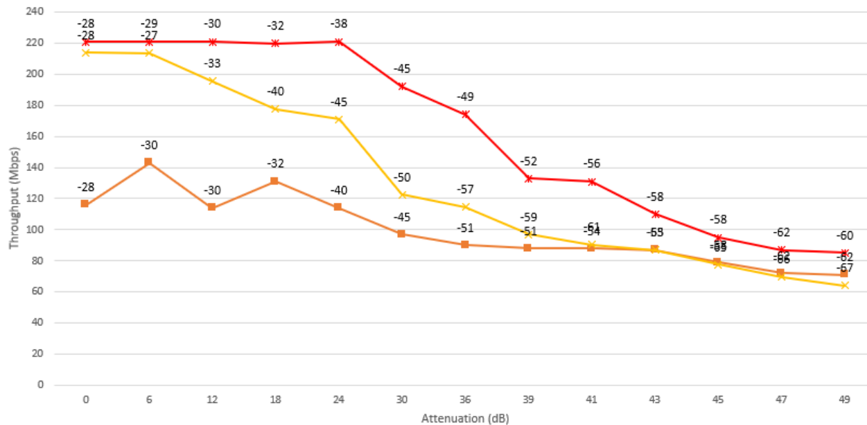
Band 2.4GHz: Upload (Mbps) - STA 802.11AX 20MHz
