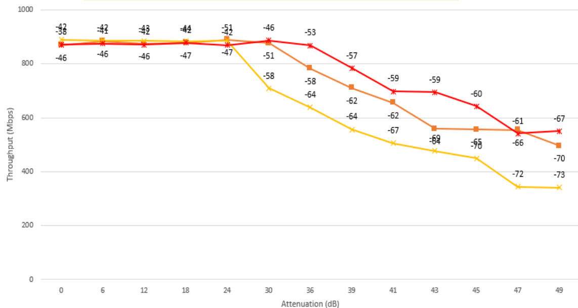
Band 5GHz: Download (Mbps) - STA 802.11AX 80MHz
