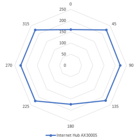
Spatial Consistency_2.4GHz_Download with STA's RSSI around -65 dBm to -70dBm
